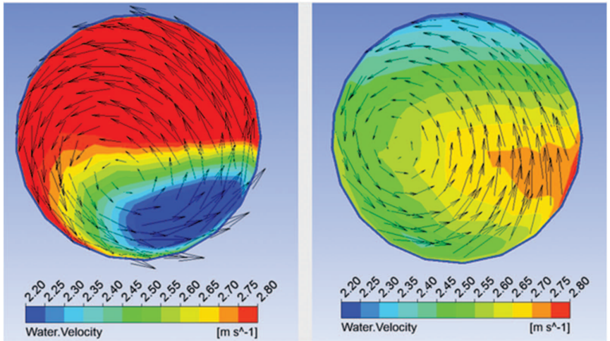
Figure 12-3. Velocity distribution examples from CFD analysis.
