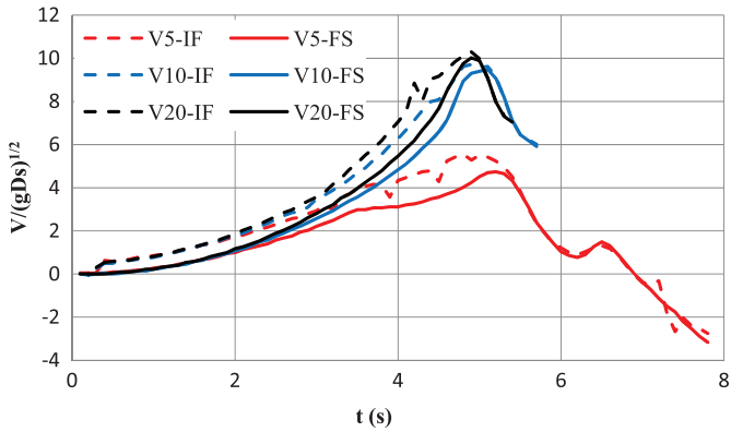
Figure 23-8. Evolution of a normalized air–water interface and water free surface velocities.
