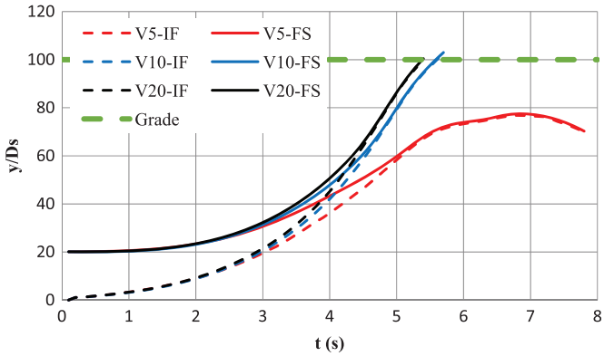
Figure 23-7. Evolution of a normalized air–water interface (IF) and water free surface (FS) displacements.
