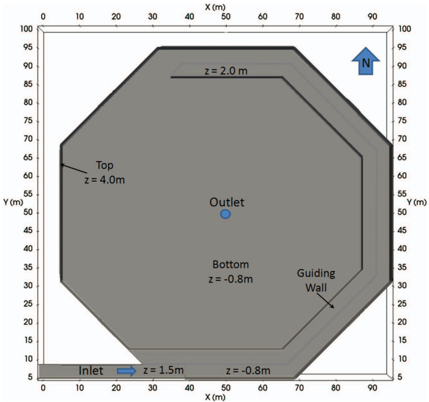
Figure 20-1. Plan view of the pond configuration.
