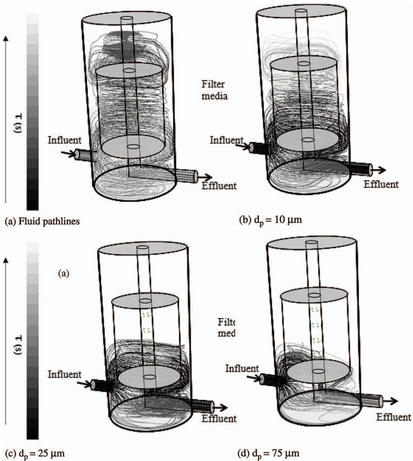
Fig. 21-5. CFD predictions of trajectories of fluid and particles inside the RCF, shaded on the basis of residence time, \tau .
